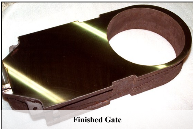
Being coated with Tungsten Carbide
