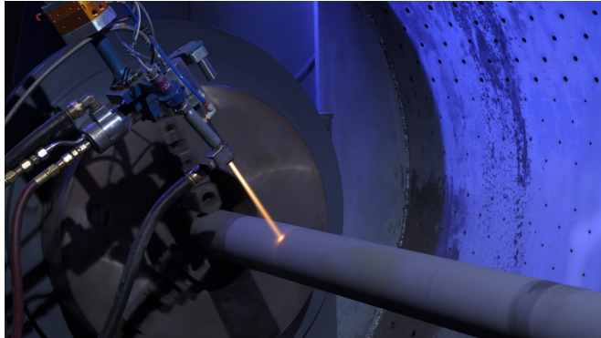
Rod being coated with tungsten carbide
